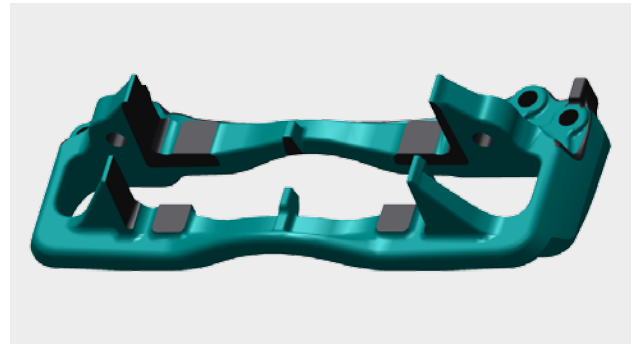
Tangential Pad Carrier
